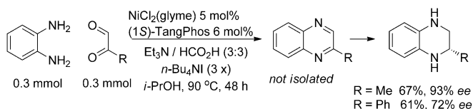
Scheme 5. Asymmetric reductive amination of 1,2-diaminobenzene with \alpha -ketoaldehydes (0.3 mmol scale).
