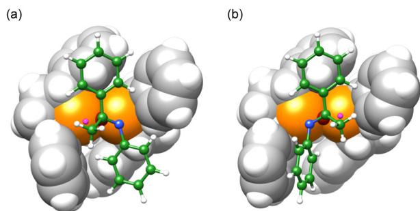
Figure 1. Transition-state structures TS-S (a) and TS-R (b) for hydride insertion of cationic [(R)-Ph-BPE](hydrido)nickel(II) into a \pi -bound N -phenylketimine to give the major (S) and minor (R) isomers, respectively (see Scheme 6a). The ligand Ph-BPE is shown in space-filling mode while other molecules are shown as ball-and-stick models. Nickel is shown in dark red, hydride in pink, phosphorus in orange, nitrogen in blue, and carbon atoms of the ketimine in green.
