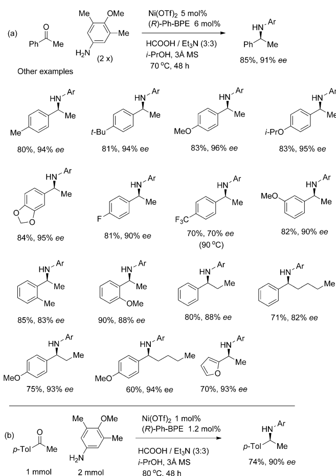
Scheme 3. Asymmetric reductive amination of aromatic ketones with 3,5-dimethylanisidine (0.3 mmol scale in most cases).
