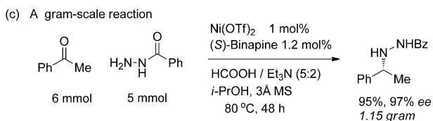
Scheme 4. Asymmetric reductive amination of ketones with benzhydrazide (0.3 mmol scale in most cases).
