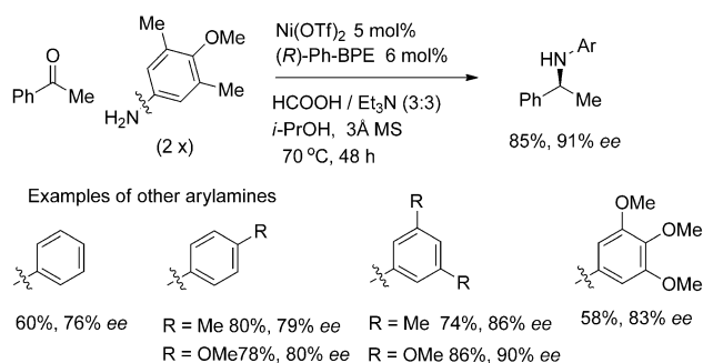
Scheme 2. Asymmetric reductive amination of acetophenone with several anilines (0.3 mmol scale).
