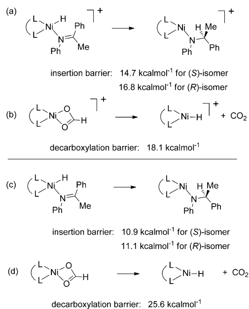
Scheme 6. Calculations on both steps of hydride insertion and decarboxylation in nickel catalysis where L–L is ( R )-Ph-BPE.
