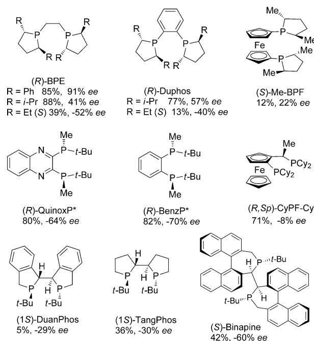
Scheme 1. The effect of chiral bisphosphines in a model reductive amination of 3,5-dimethyl-4-anisidine and acetophenone (0.1 mmol scale).
